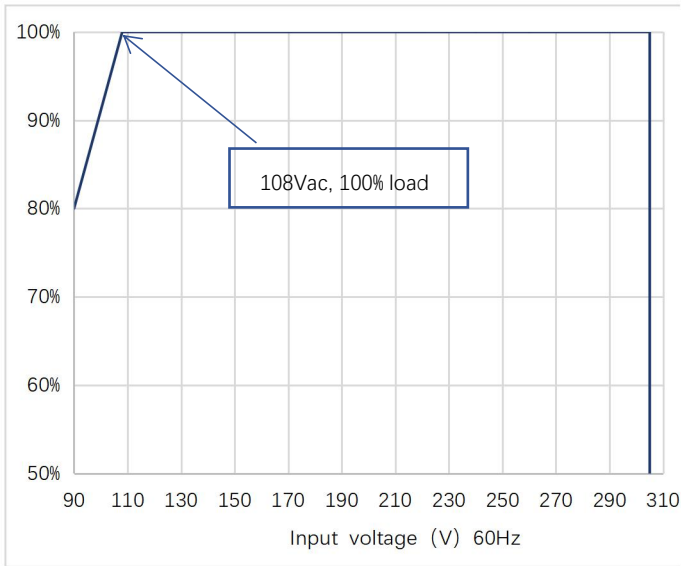
Load Derating Curve
